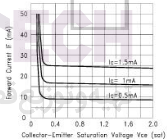
Fig.4 FORWARD CURRENT VS. COLLECTOR-EMITTER SATURATION VOLTAGE
